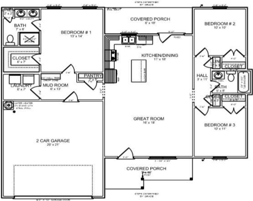
FLOOR PLAN
